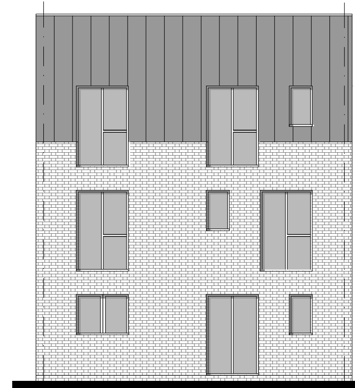
Rear Elevation
