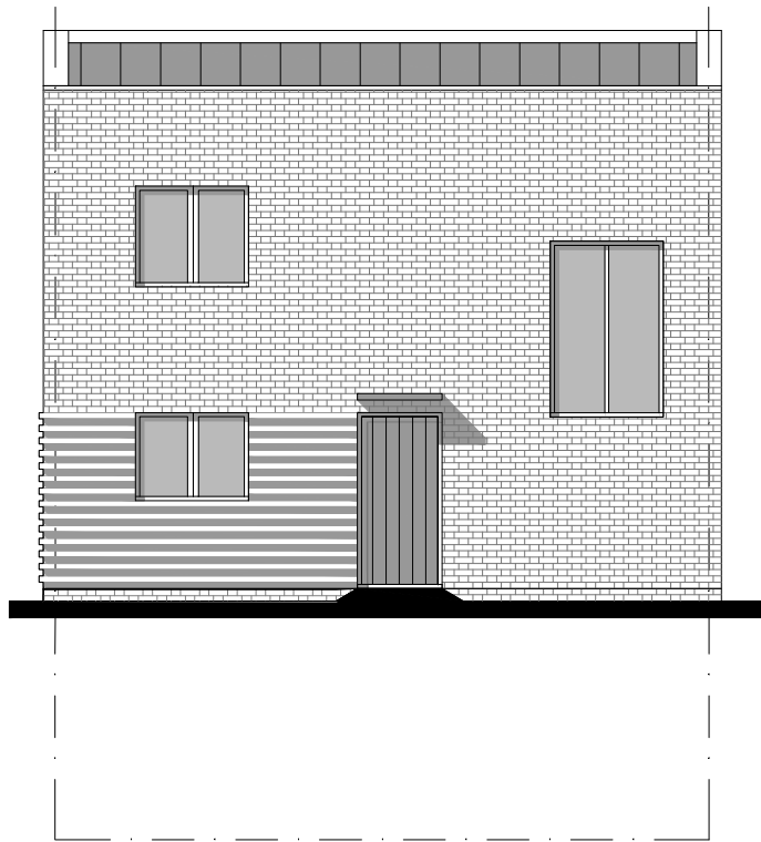
Front Elevation (Type 1)
