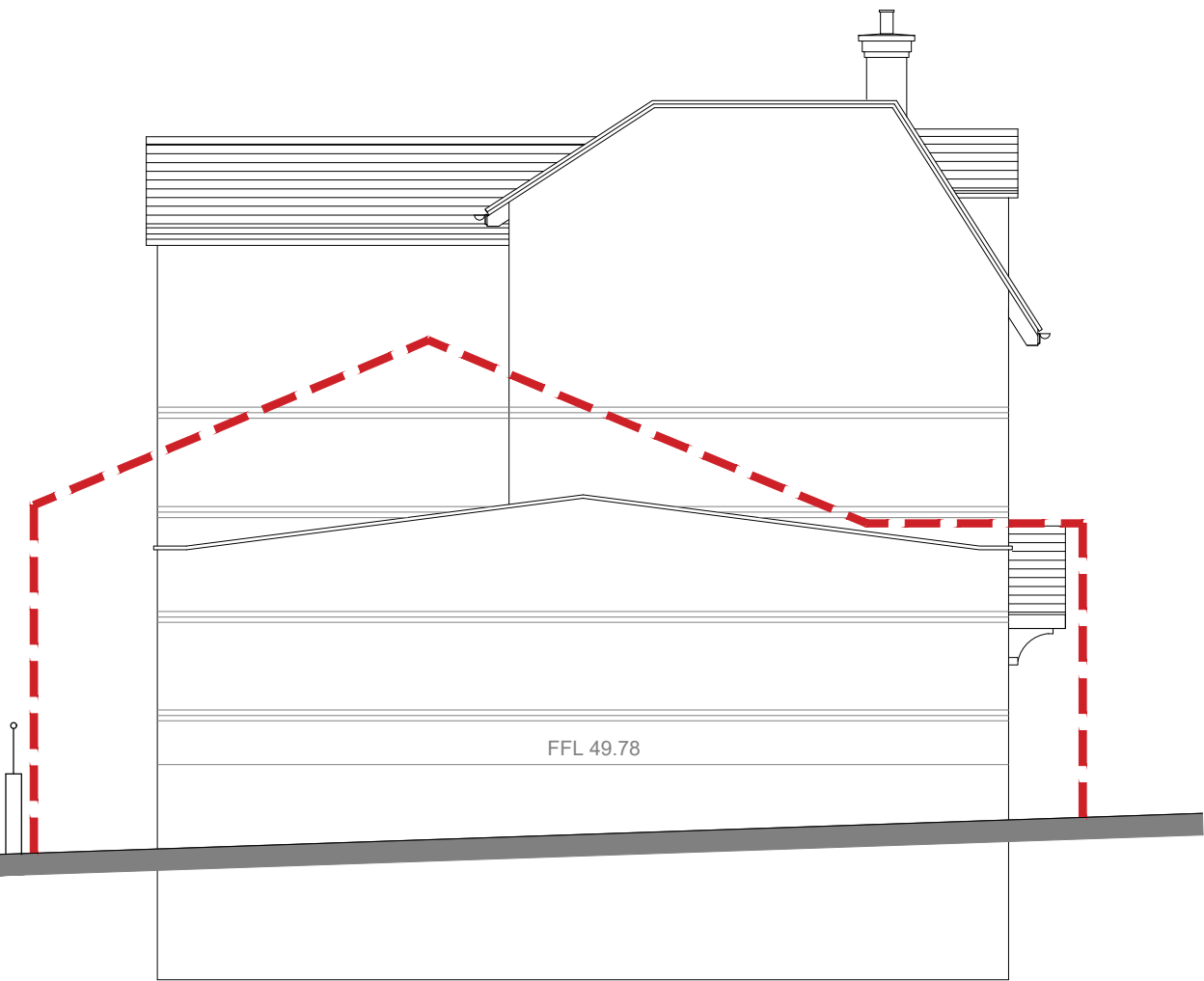
SIDE ELEVATION
