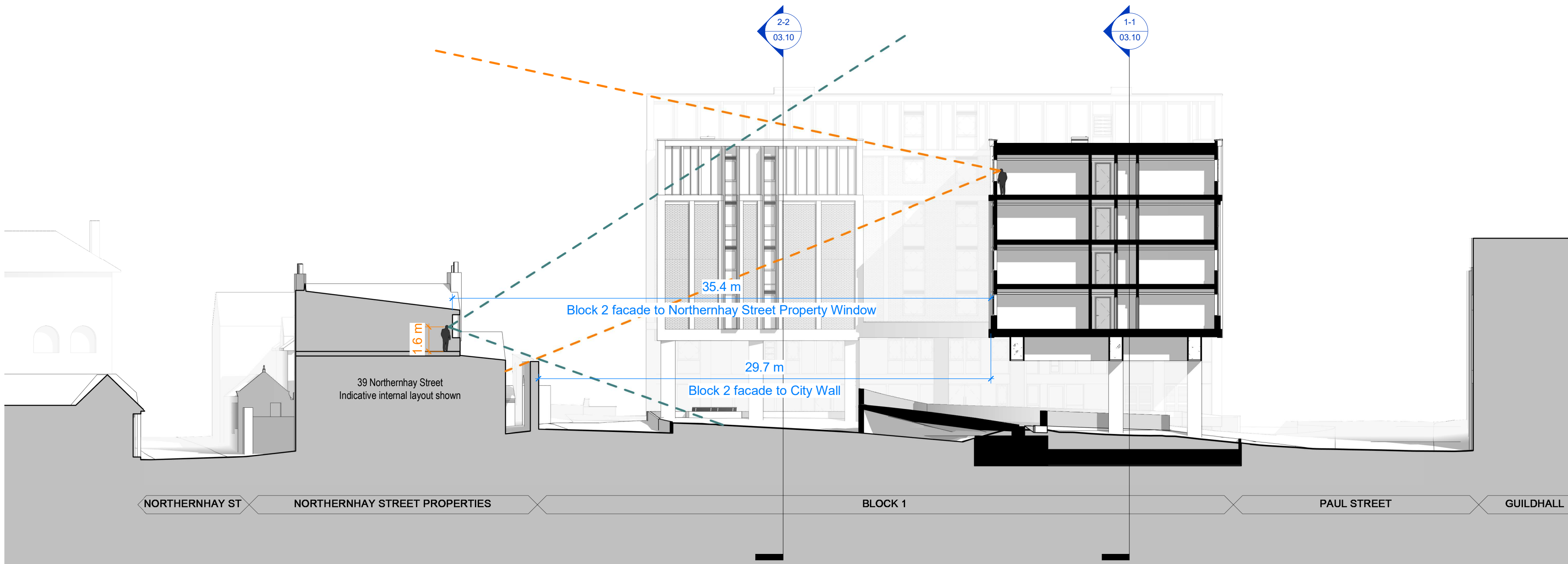
Proposed Site Section L-L 1 : 200
