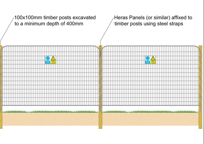
Tree Protection Fencing Specification
