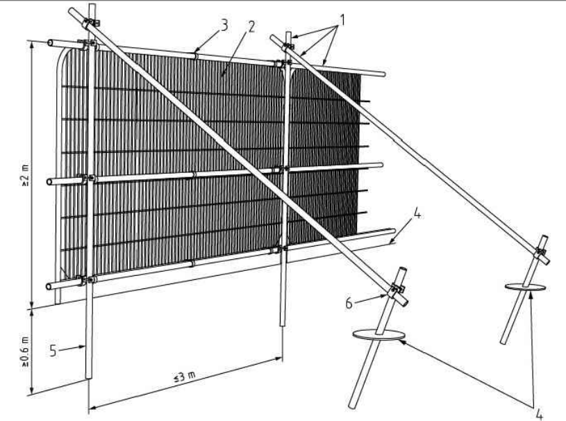
Tree Protection Fencing Specification
