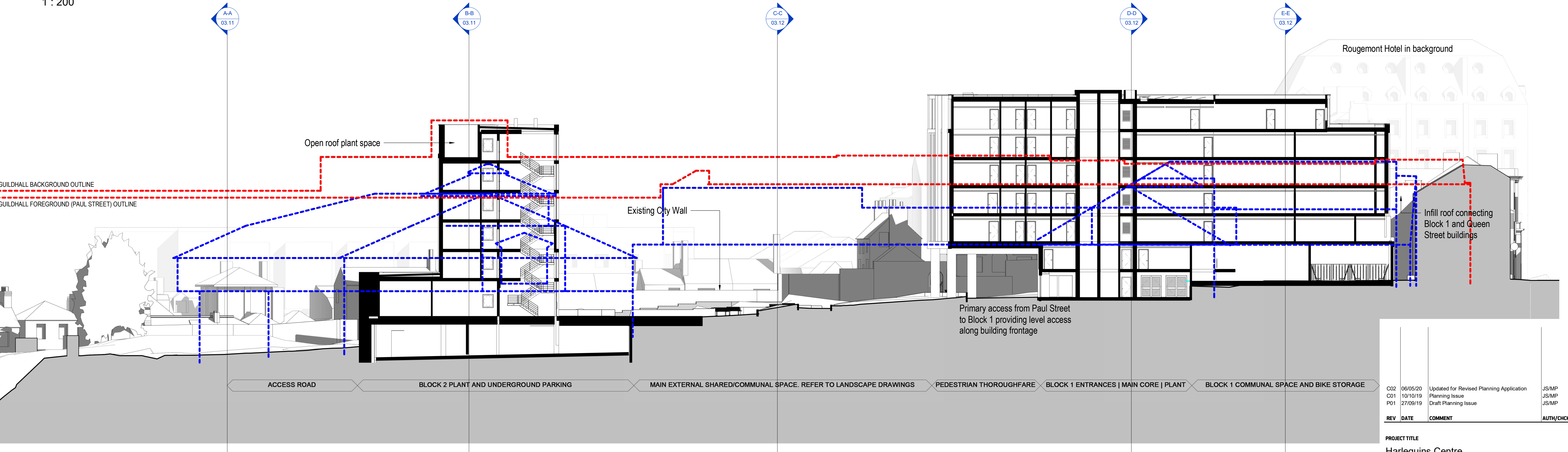
Proposed Site Section 2-2 1 : 200
