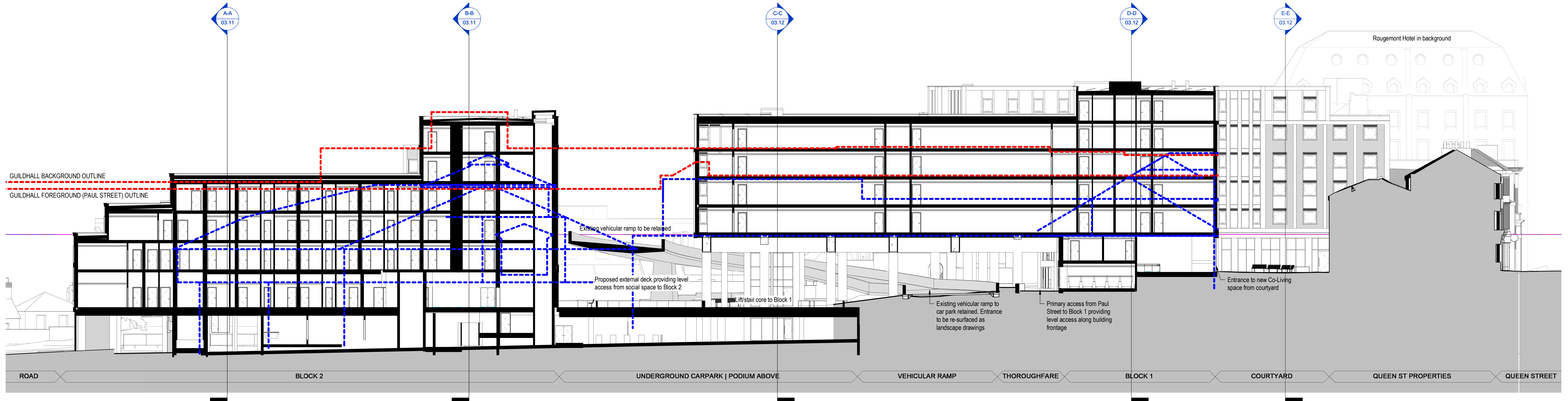
Proposed Site Section 1-1 1 : 200
